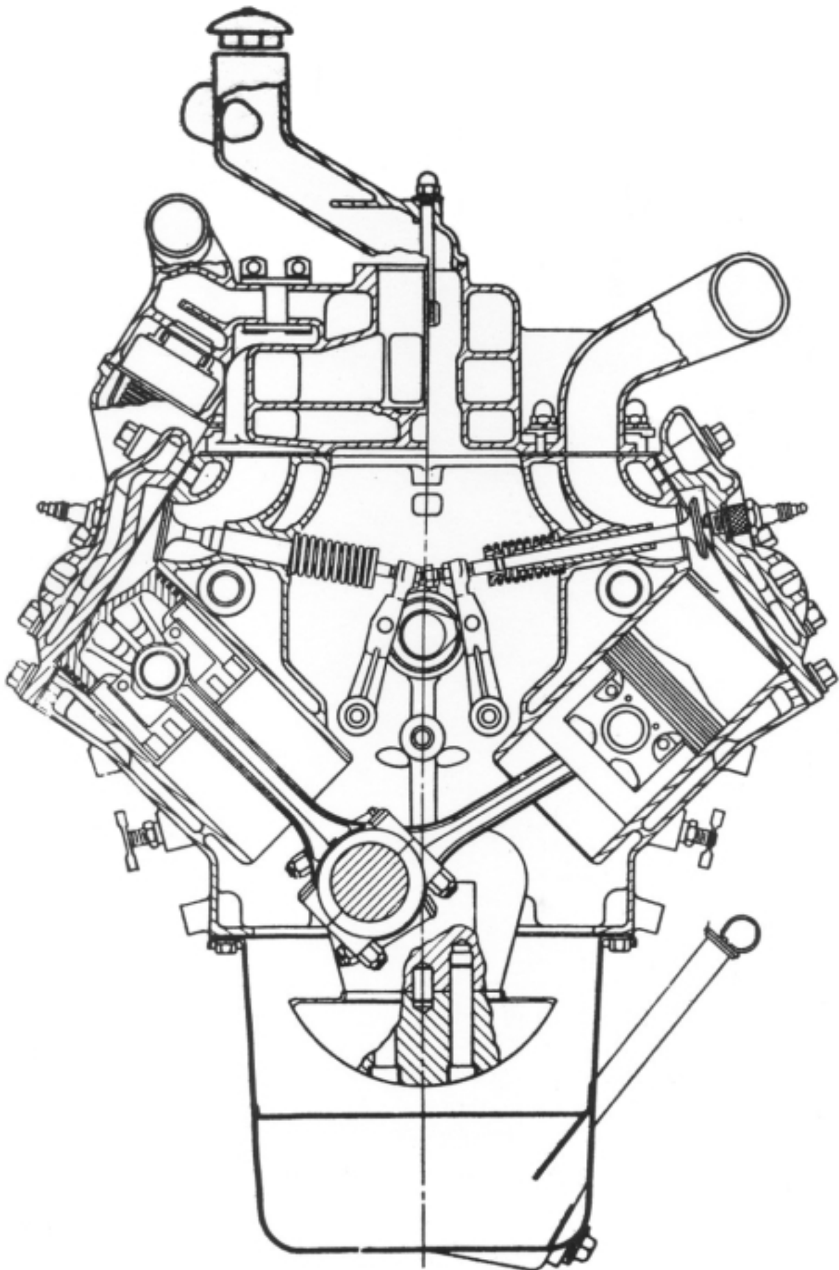
LYCOMING V-TYPE EIGHT-CYLINDER ENGINE, MODEL FB Used exclusively in 1936 and 1937 Cord automobiles
