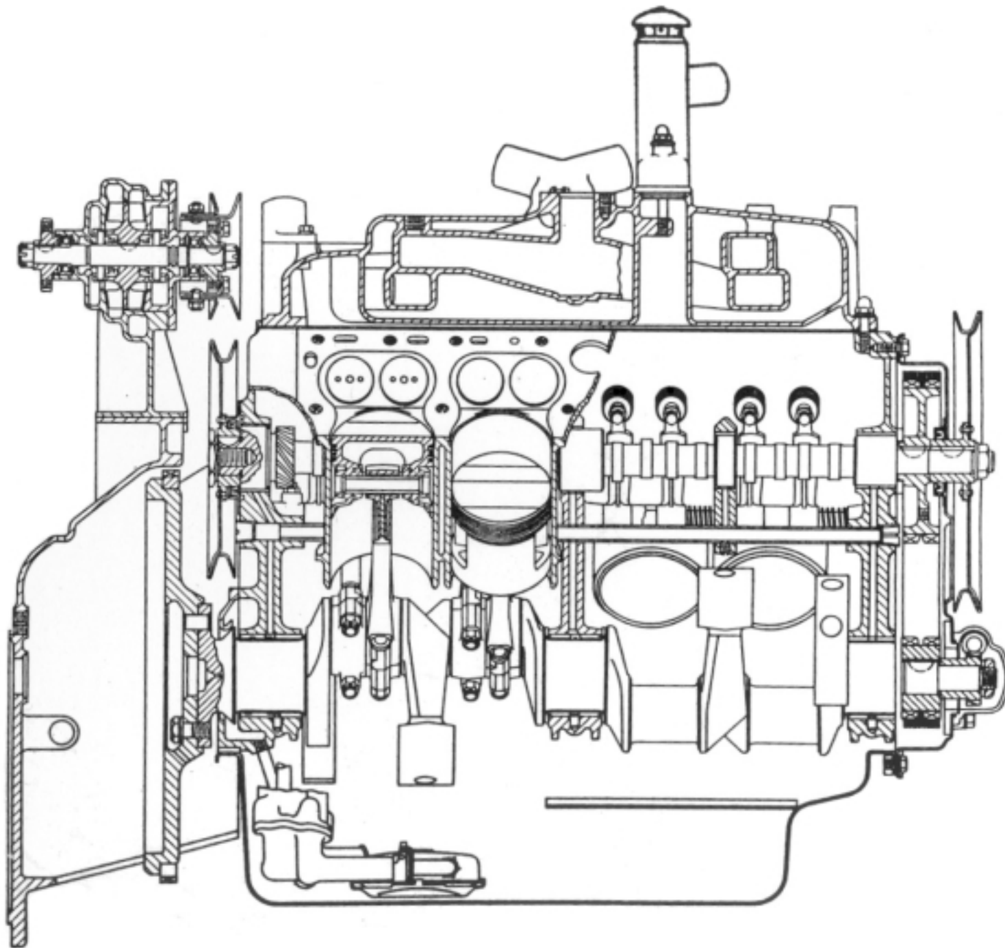
LYCOMING V-TYPE EIGHT-CYLINDER ENGINE, MODEL FB Used exclusively in 1936 and 1937 Cord automobiles
